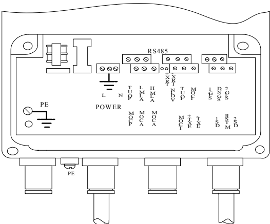
Fig.4.3 (a) Connectors for 211B
